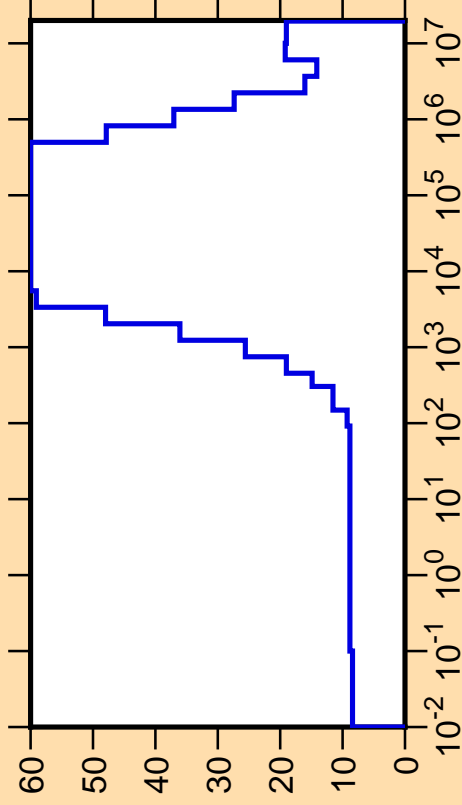
\Delta\mu/\mu vs. E for ^{114}\text{Ag}(\text{mt251})
