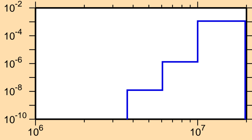
\sigma vs. E for ^{114}\text{Ag}(n,\alpha)
