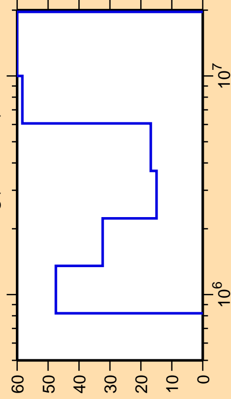
\Delta\sigma/\sigma vs. E for ^{114}\text{Ag}(n,ncont.)
