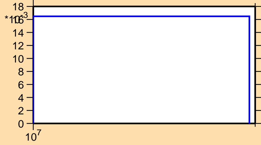
\sigma vs. E for ^{114}\text{Ag}(n,3n)
