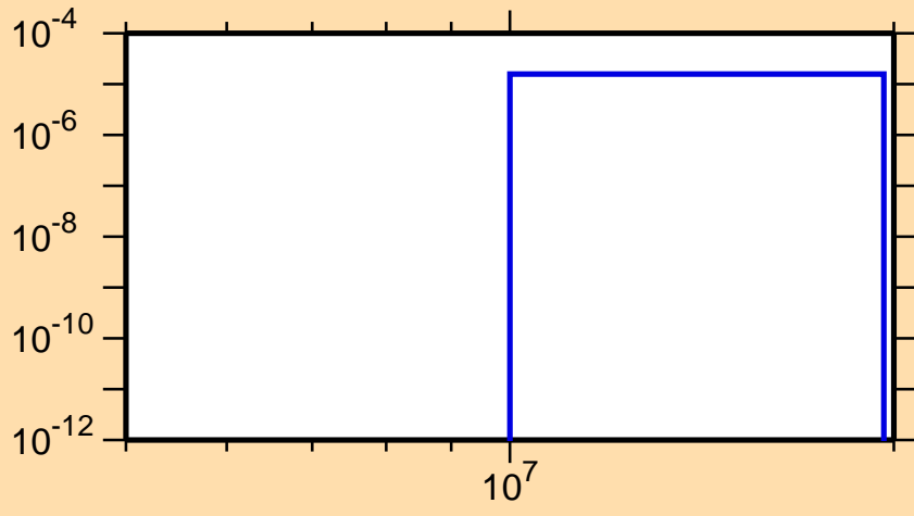
\sigma vs. E for ^{114}\text{Ag}(n,n\alpha)
