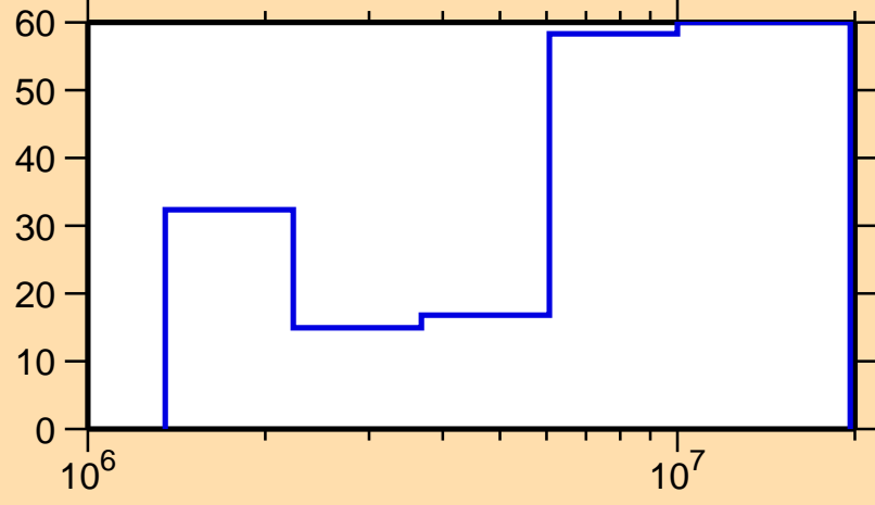
\Delta\sigma/\sigma vs. E for ^{114}\text{Ag}(n,n\text{cont.})
