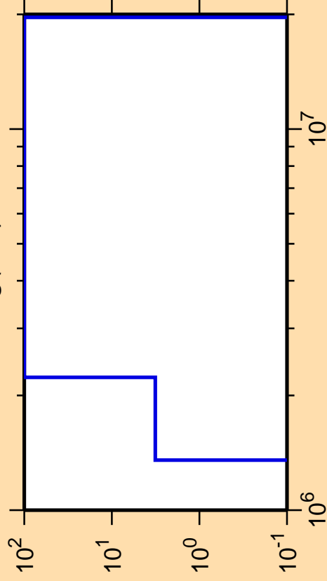
\Delta\sigma/\sigma vs. E for ^{114}\text{Ag}(n,\alpha)
