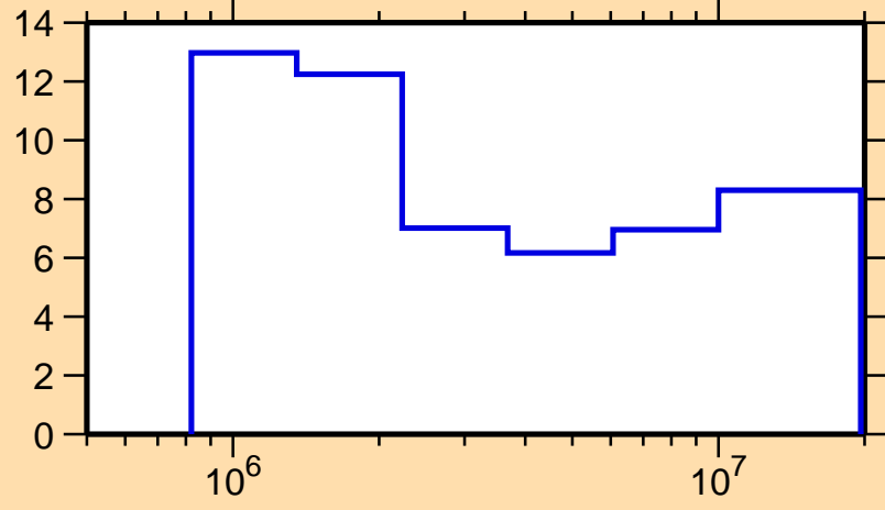
\Delta\sigma/\sigma vs. E for ^{114}\text{Ag}(n,nonel.)
