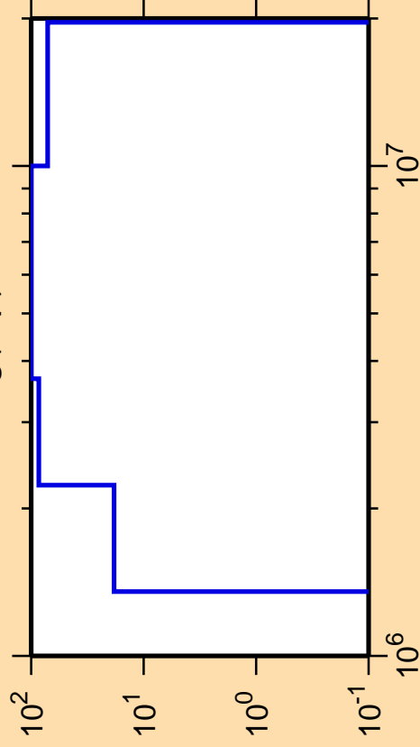
\Delta\sigma/\sigma vs. E for ^{114}\text{Ag}(n,p)
