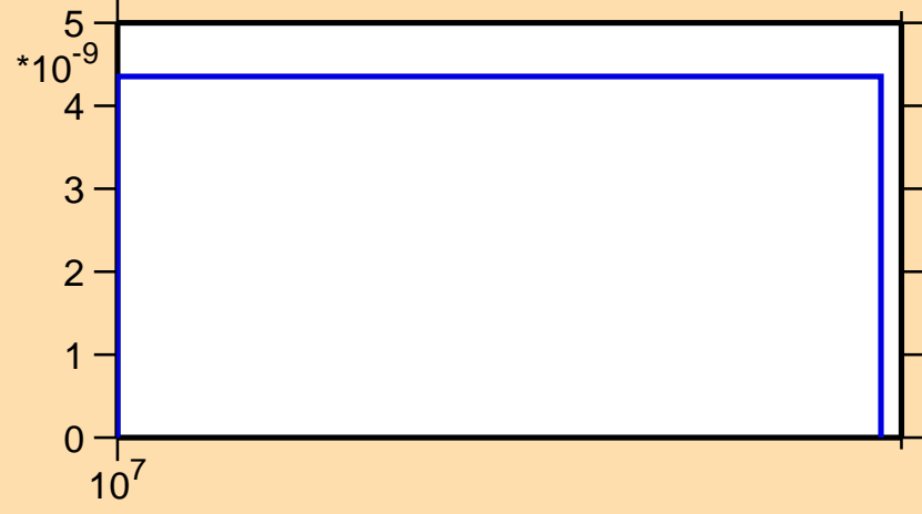
\sigma vs. E for ^{114}\text{Ag}(n,nt)
