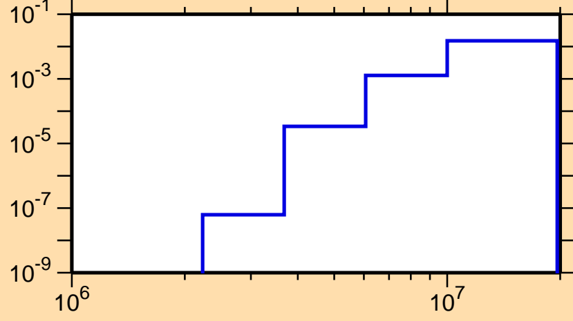
\sigma vs. E for ^{114}\text{Ag}(n,p)
