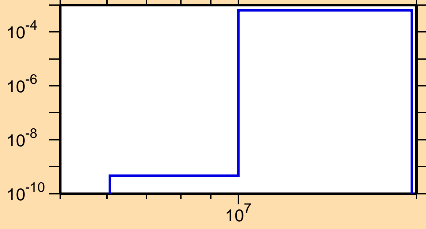
\sigma vs. E for ^{114}\text{Ag}(n,d)
