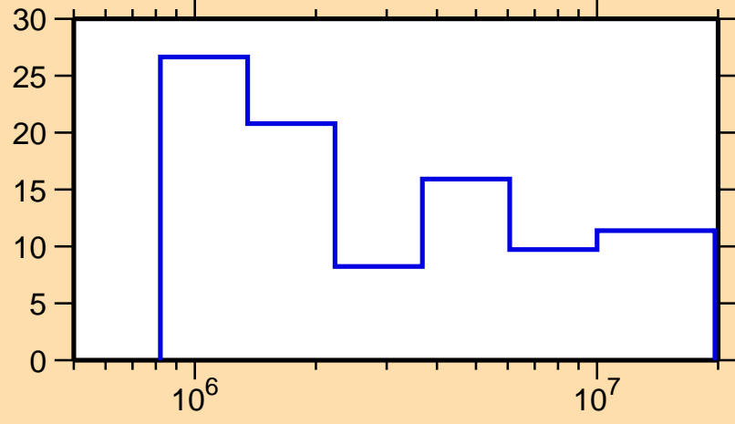
\Delta\sigma/\sigma vs. E for ^{114}\text{Ag}(n,tot.)
