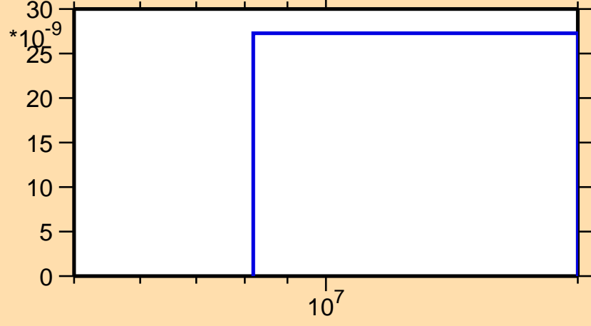
\sigma vs. E for ^{114}\text{Ag}(n,2np)
