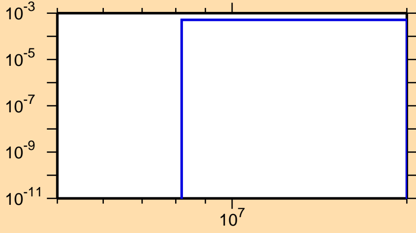
\sigma vs. E for ^{114}\text{Ag}(n,d)
