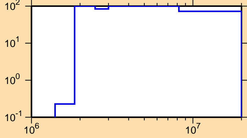
\Delta\sigma/\sigma vs. E for ^{114}\text{Ag}(n,p)
