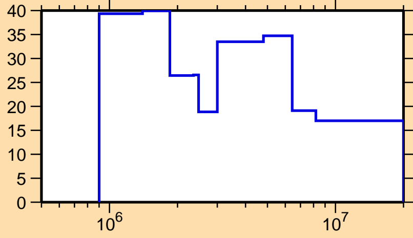
\Delta\sigma/\sigma vs. E for ^{114}\text{Ag}(n,el.)
