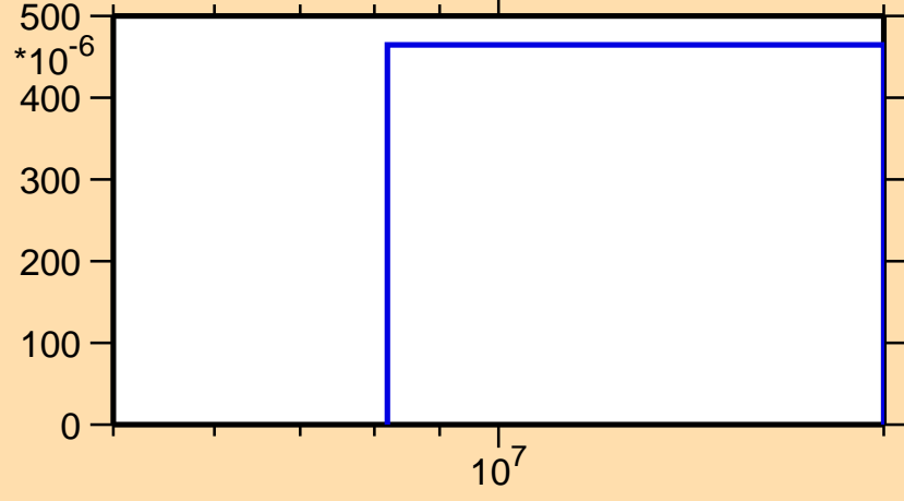
\sigma vs. E for ^{114}\text{Ag}(n,np)
