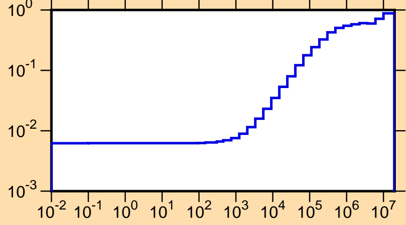
\mu vs. E for ^{115}\text{Ag}(\text{mt251})
