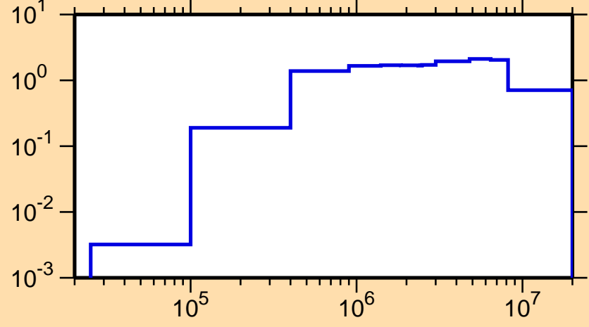
\sigma vs. E for ^{115}\text{Ag}(n,\text{inel.})
