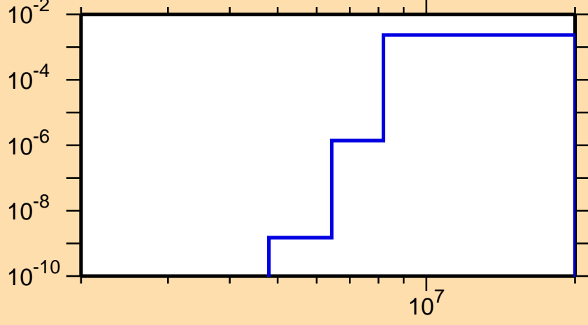
\sigma vs. E for ^{115}\text{Ag}(n,p)
