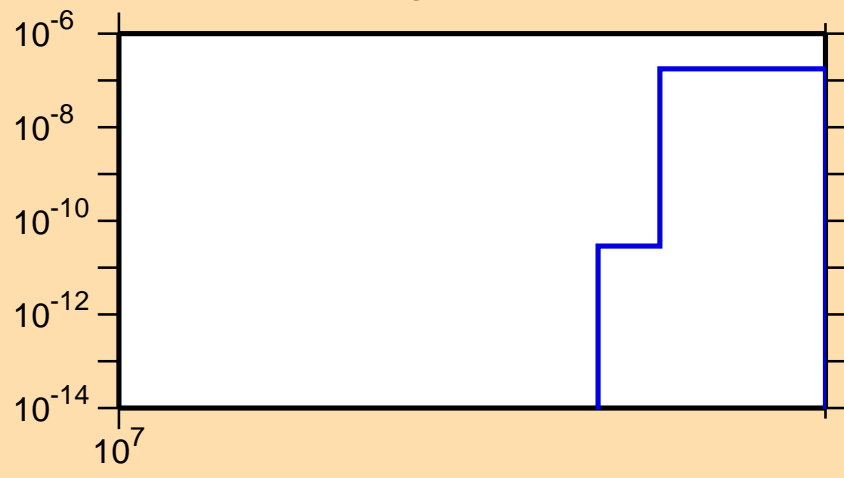
\sigma vs. E for ^{115}\text{Ag}(n,\text{nd})
