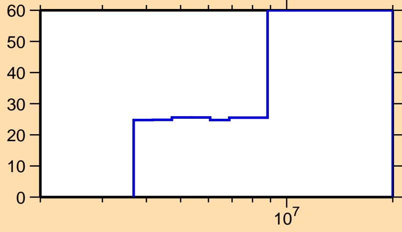
\Delta\sigma/\sigma vs. E for ^{115}\text{Ag}(n,ncont.)
