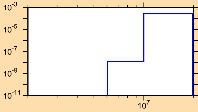
\sigma vs. E for ^{115}\text{Ag}(n,\alpha)
