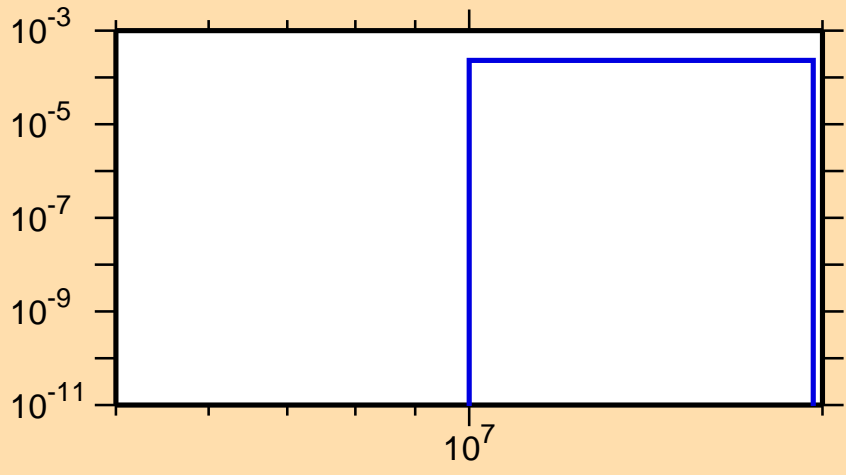
\sigma vs. E for ^{115}\text{Ag}(n,d)
