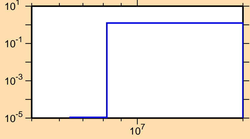
\sigma vs. E for ^{115}\text{Ag}(n,2n)
