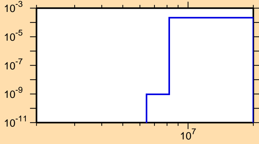
\sigma vs. E for ^{115}\text{Ag}(n,\alpha)
