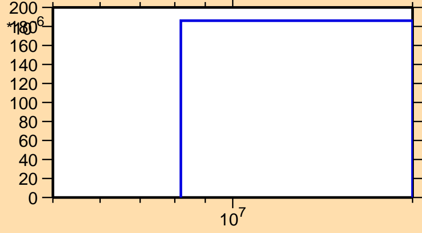
\sigma vs. E for ^{115}\text{Ag}(n,d)
