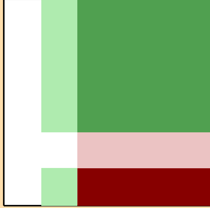
\Delta\sigma/\sigma vs. E for ^{115}\text{Ag}(n,2n)
