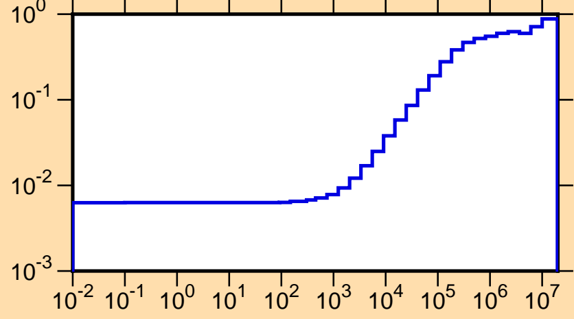
\mu vs. E for ^{116}\text{Ag}(\text{mt251})
