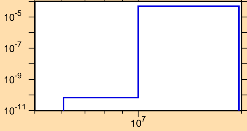
\sigma vs. E for ^{116}\text{Ag}(n,t)
