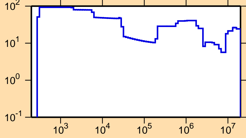
\Delta\sigma/\sigma vs. E for ^{116}\text{Ag}(n,\text{tot.})
