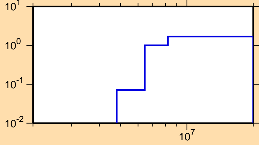
\sigma vs. E for ^{116}\text{Ag}(n,2n)
