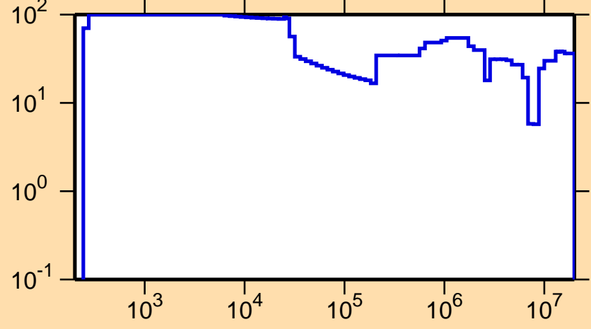
\Delta\sigma/\sigma vs. E for ^{116}\text{Ag}(n,\text{el.})
