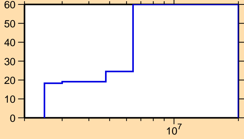
\Delta\sigma/\sigma vs. E for ^{116}\text{Ag}(n,ncont.)
