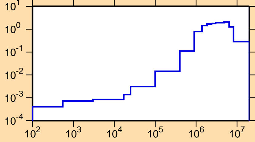
\sigma vs. E for ^{116}\text{Ag}(n,\text{inel.})
