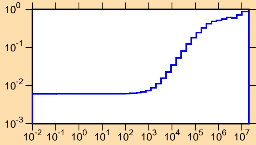
\mu vs. E for ^{117}\text{Ag}(\text{mt251})
