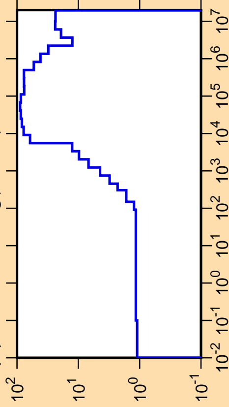
\Delta\mu/\mu vs. E for ^{117}\text{Ag}(\text{mt251})
