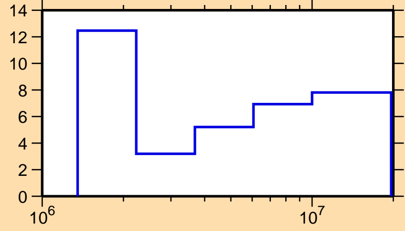
\Delta\sigma/\sigma vs. E for ^{117}\text{Ag}(n,n\text{onel.})
