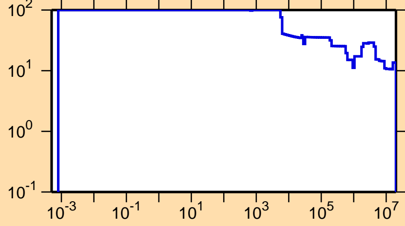
\Delta\sigma/\sigma vs. E for ^{118}\text{Ag}(n,\text{el.})
