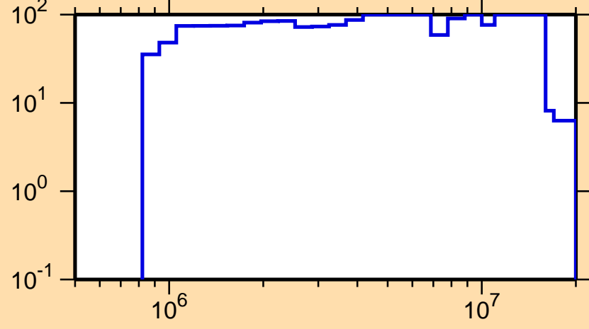
\Delta\sigma/\sigma vs. E for ^{118}\text{Ag}(n,n_1)
