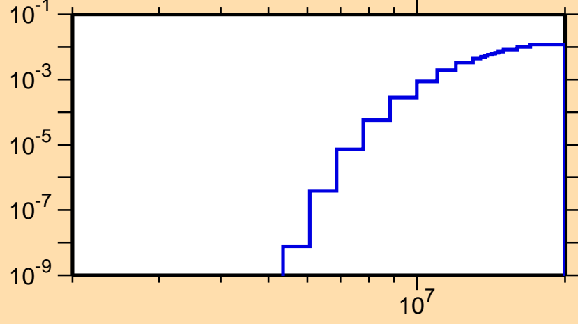
\sigma vs. E for ^{118}\text{Ag}(n,p)
