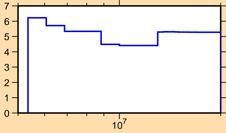
\Delta\sigma/\sigma vs. E for ^{118}\text{Ag}(n,\text{nonel.})
