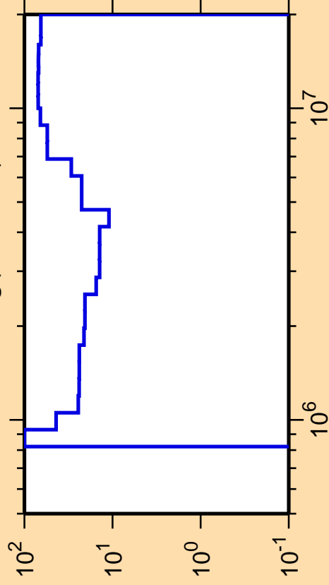
\Delta\sigma/\sigma vs. E for ^{118}\text{Ag}(n,\text{ncont.})
