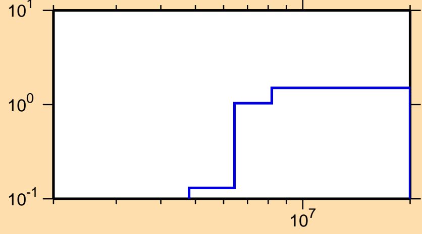
\sigma vs. E for ^{118}\text{Ag}(n,2n)
