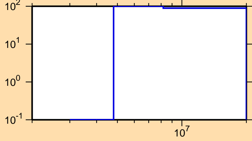
\Delta\sigma/\sigma vs. E for ^{118}\text{Ag}(n,p)
