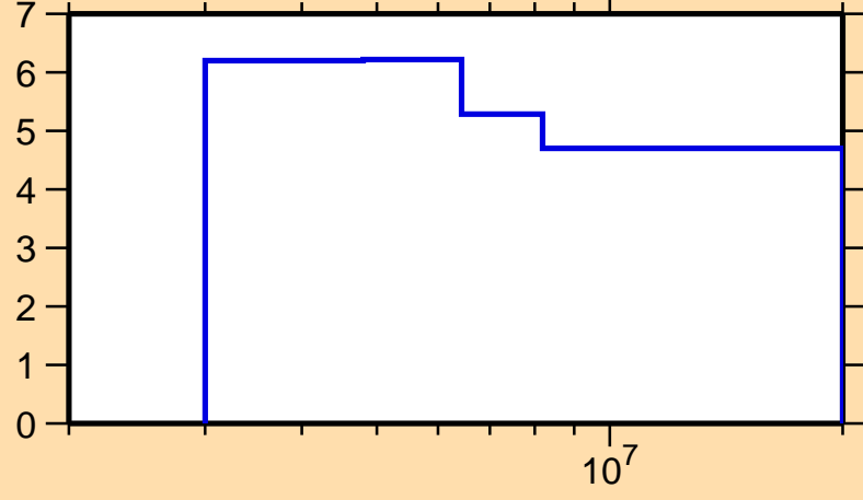
\Delta\sigma/\sigma vs. E for ^{118}\text{Ag}(n,\text{nonel.})
