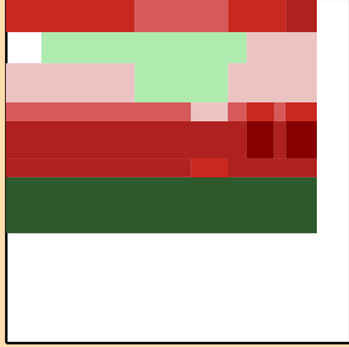
\Delta\sigma/\sigma vs. E for ^{118}\text{Ag}(n,n_1)
