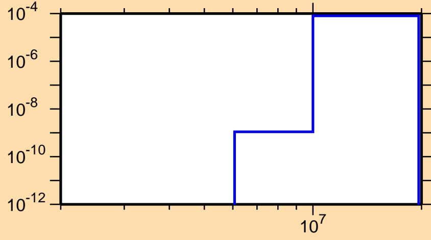
\sigma vs. E for ^{118}\text{Ag}(n,\alpha)
