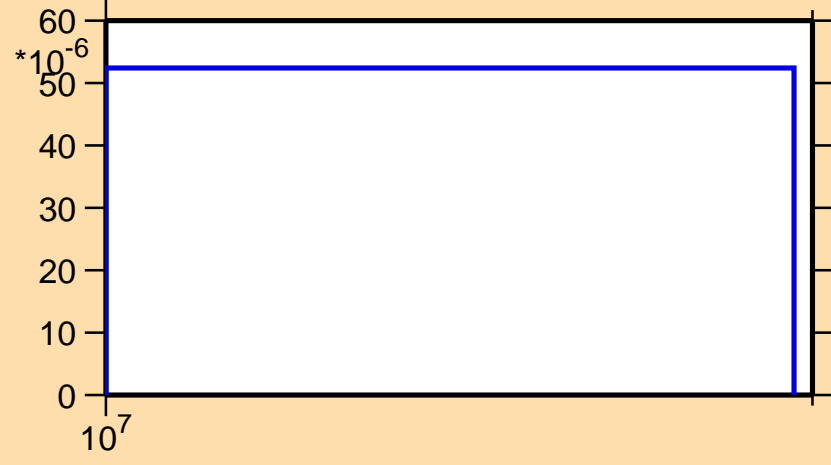
\sigma vs. E for ^{118}\text{Ag}(n,np)
