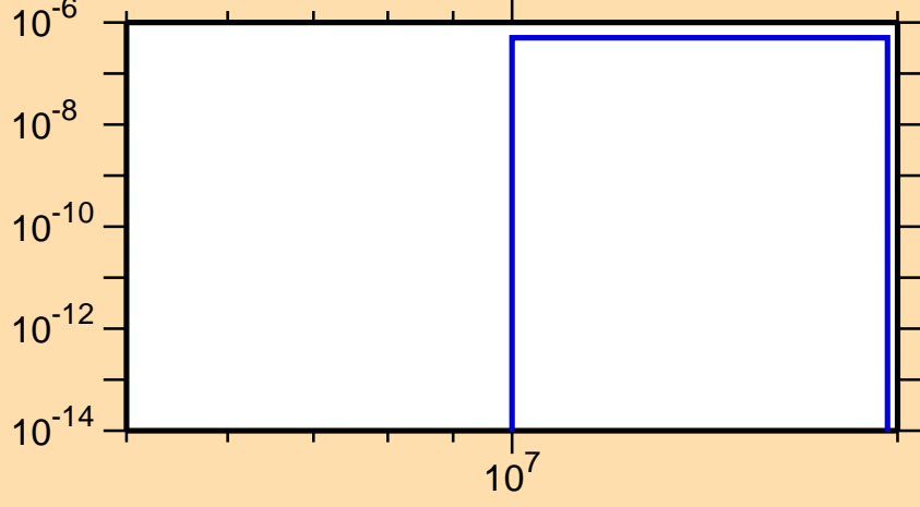
\sigma vs. E for ^{118}\text{Ag}(n,n\alpha)
