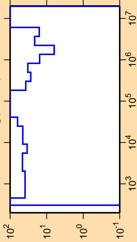
\Delta\sigma/\sigma vs. E for ^{118}\text{Ag}(n,\text{inel.})
