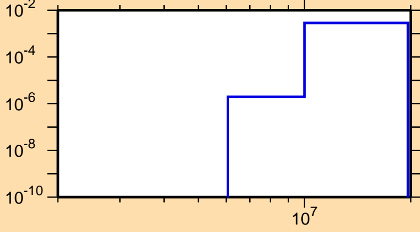
\sigma vs. E for ^{118}\text{Ag}(n,p)
