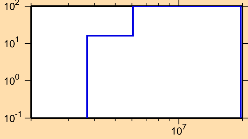
\Delta\sigma/\sigma vs. E for ^{118}\text{Ag}(n,ncont.)
