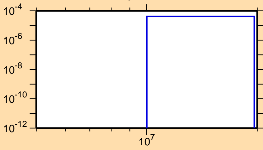
\sigma vs. E for ^{118}\text{Ag}(n,d)
