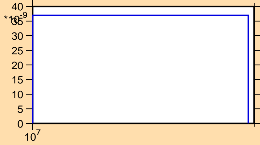
\sigma vs. E for ^{118}\text{Ag}(n,\text{nd})
