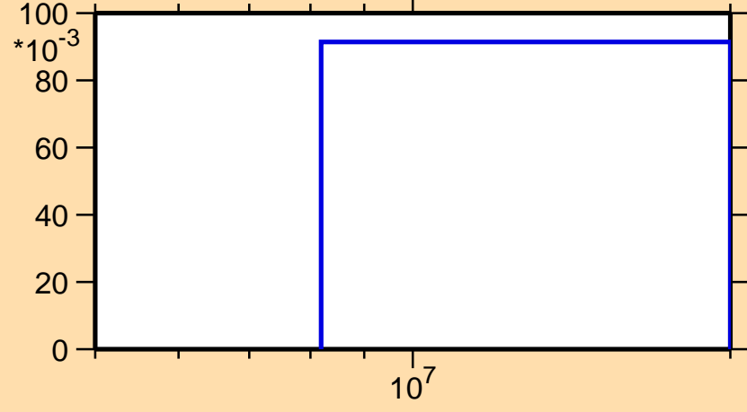
\sigma vs. E for ^{118}\text{Ag}(n,3n)
