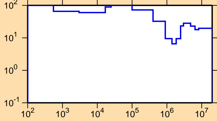
\Delta\sigma/\sigma vs. E for ^{118}\text{Ag}(n,\text{nonel.})
