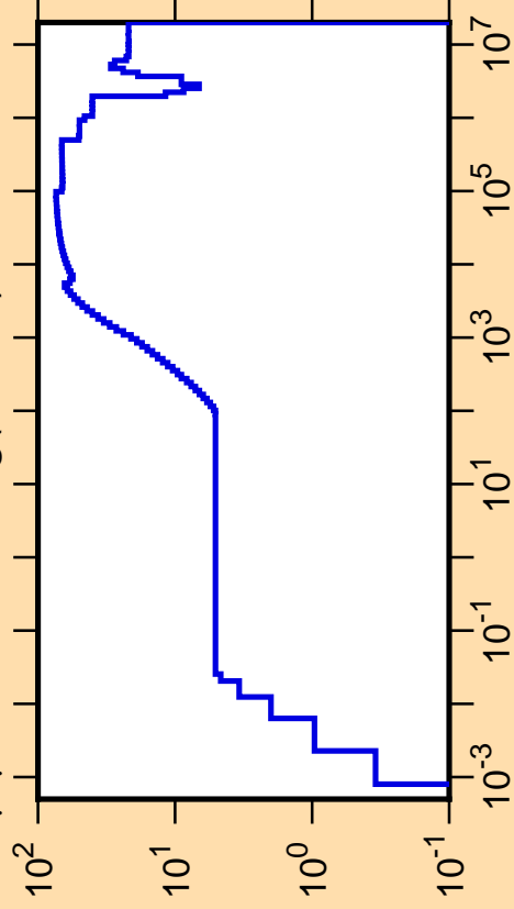
\Delta\mu/\mu vs. E for ^{119}\text{Ag}(\text{mt251})
