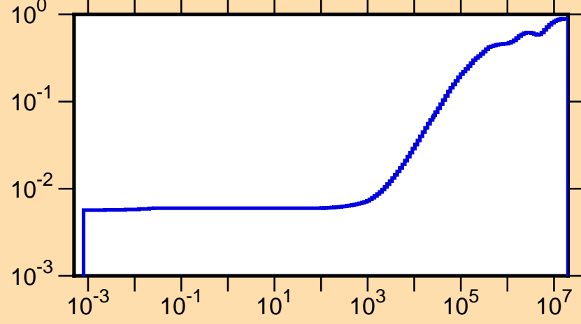
\mu vs. E for ^{119}\text{Ag}(\text{mt251})
