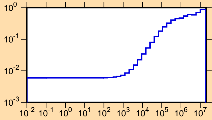
\mu vs. E for ^{119}\text{Ag}(\text{mt251})
