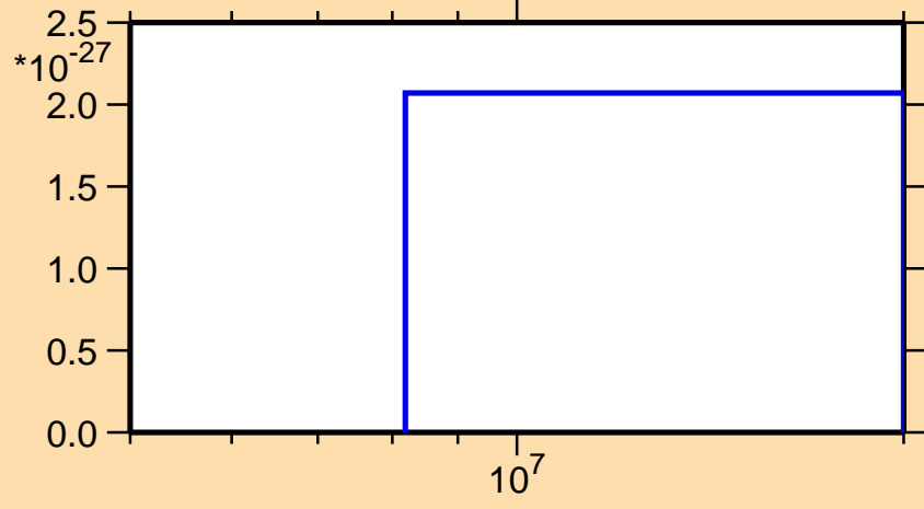
\sigma vs. E for ^{119}\text{Ag}(\text{mt } 11)
