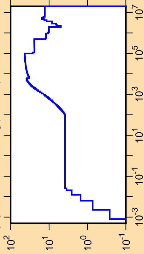
\Delta\mu/\mu vs. E for ^{120}\text{Ag}(\text{mt251})
