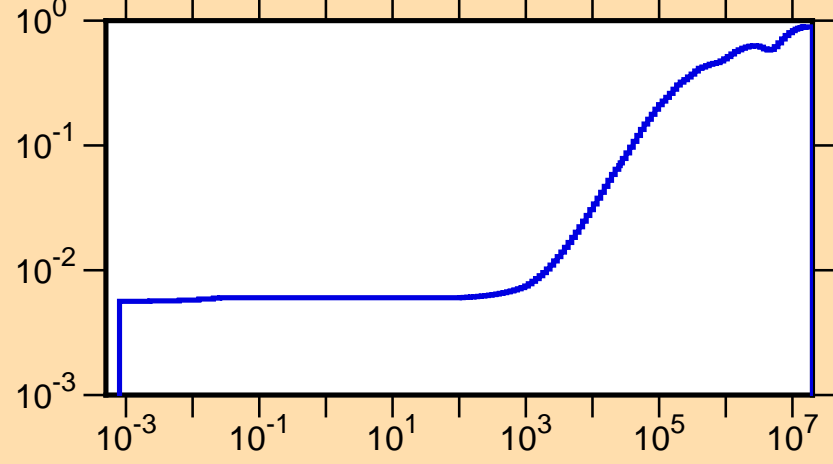
\mu vs. E for ^{120}\text{Ag}(\text{mt251})
