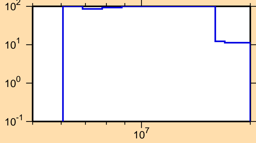
\Delta\sigma/\sigma vs. E for ^{120}\text{Ag}(n,n_1)
