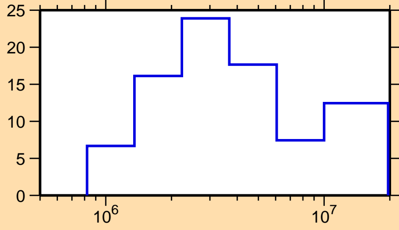
\Delta\sigma/\sigma vs. E for ^{120}\text{Ag}(n,el.)
