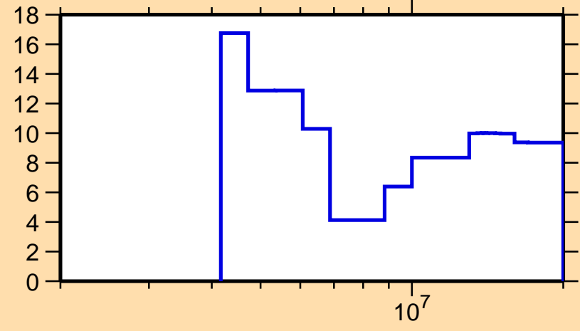
\Delta\sigma/\sigma vs. E for ^{24}\text{Al}(n,el.)
