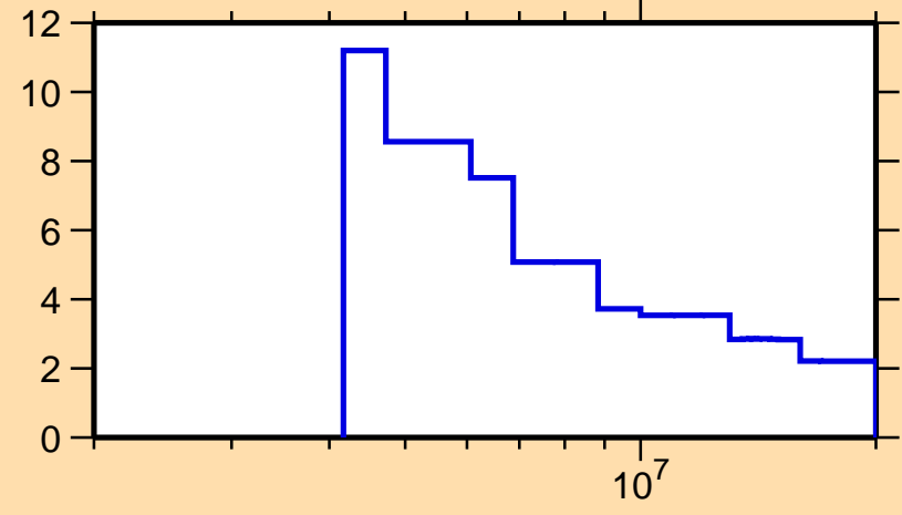
\Delta\sigma/\sigma vs. E for ^{24}\text{Al}(n,tot.)
