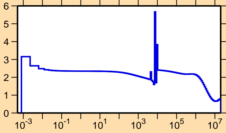
\sigma vs. E for ^{24}\text{Al}(n,\text{el.})
