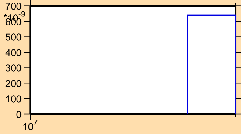
\sigma vs. E for ^{25}\text{Al}(n,\text{nd})
