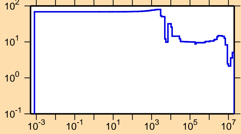
\Delta\sigma/\sigma vs. E for ^{25}\text{Al}(n,\text{el.})
