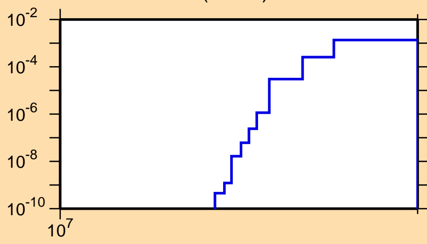
\sigma vs. E for ^{25}\text{Al}(\text{mt } 45)
