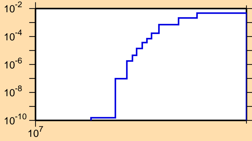
\sigma vs. E for ^{25}\text{Al}(n,pd)
