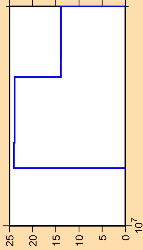
\Delta\sigma/\sigma vs. E for ^{25}\text{Al}(n,pd)
