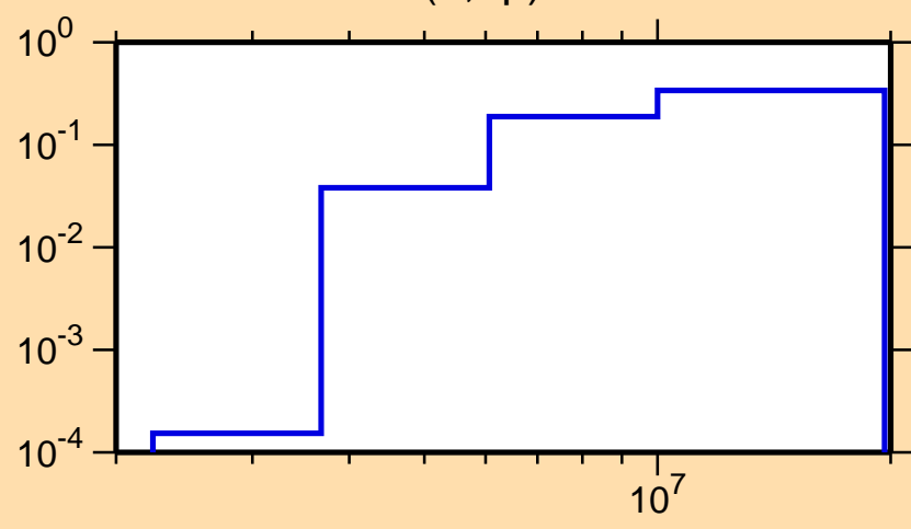
\sigma vs. E for ^{25}\text{Al}(n,np)
