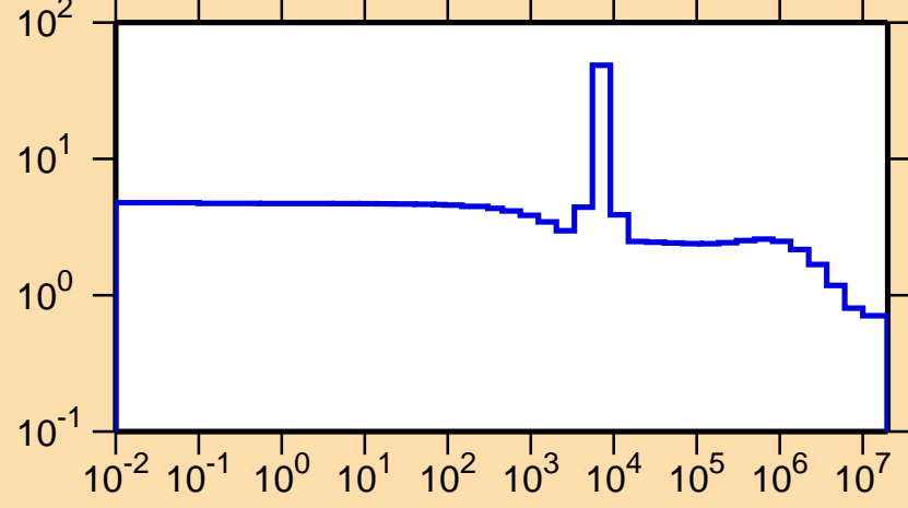
\sigma vs. E for ^{25}\text{Al}(n,\text{el.})
