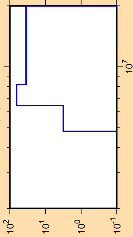
\Delta\sigma/\sigma vs. E for ^{25}\text{Al}(n,p\alpha)
