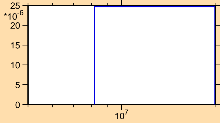
\sigma vs. E for ^{25}\text{Al}(\text{mt } 45)
