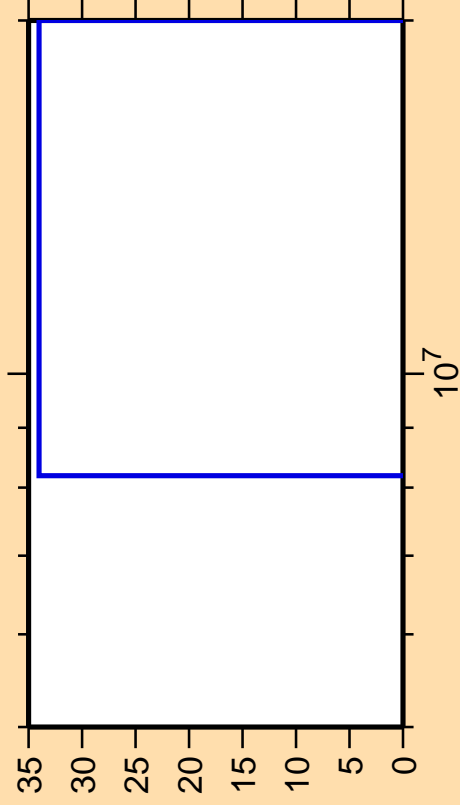
\Delta\sigma/\sigma vs. E for ^{25}\text{Al}(\text{mt } 45)
