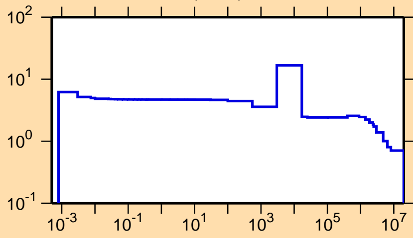
\sigma vs. E for ^{25}\text{Al}(n,\text{el.})
