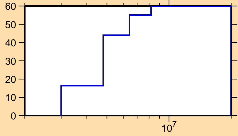
\Delta\sigma/\sigma vs. E for ^{25}\text{Al}(n,n_1)
