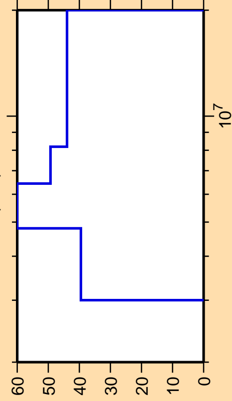
\Delta\sigma/\sigma vs. E for ^{25}\text{Al}(n,\alpha)
