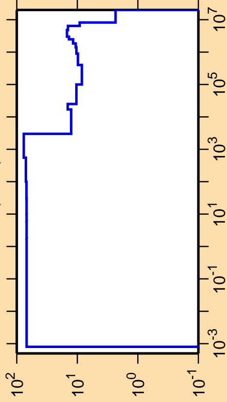
\Delta\sigma/\sigma vs. E for ^{25}\text{Al}(n,\text{el.})
