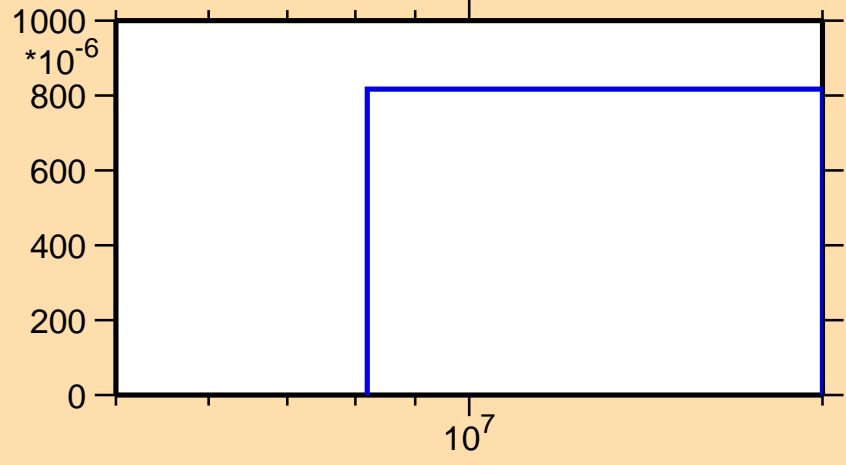
\sigma vs. E for ^{25}\text{Al}(\text{mt117})
