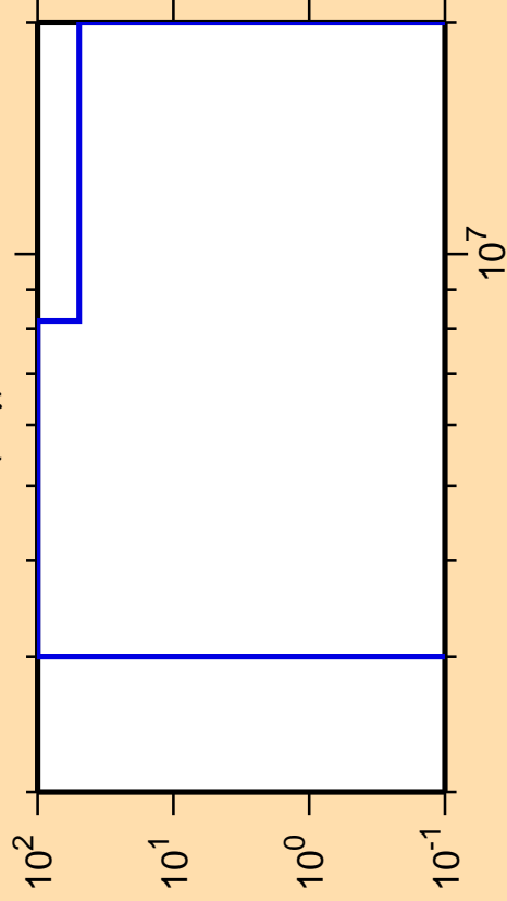
\Delta\sigma/\sigma vs. E for ^{25}\text{Al}(n,\gamma)
