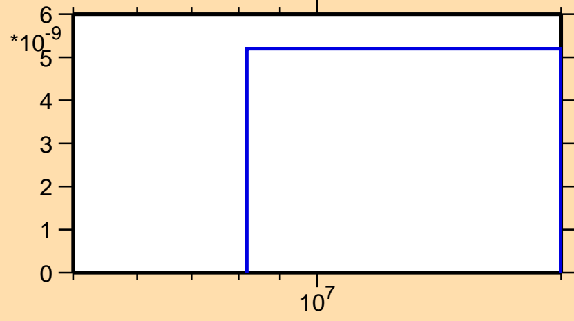
\sigma vs. E for ^{25}\text{Al}(n,nd)
