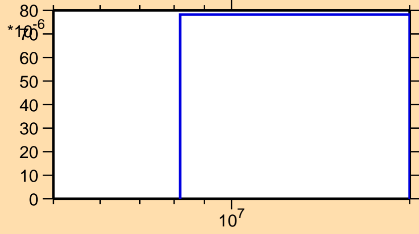
\sigma vs. E for ^{25}\text{Al}(n,t)
