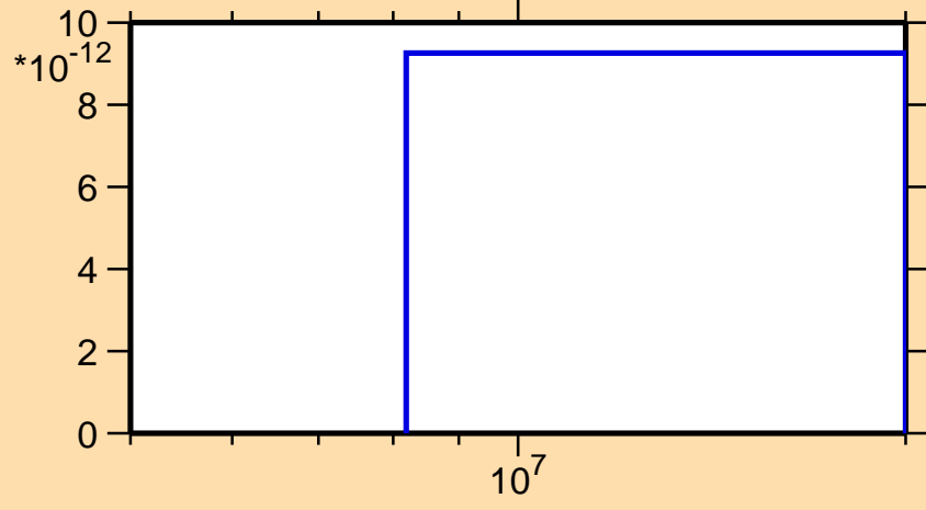
\sigma vs. E for ^{25}\text{Al}(n,\text{pt})
