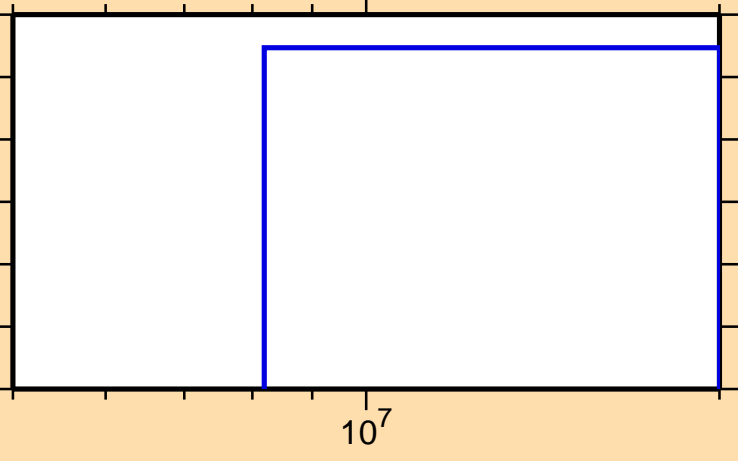
\sigma vs. E for ^{25}\text{Al}(n,2n)
