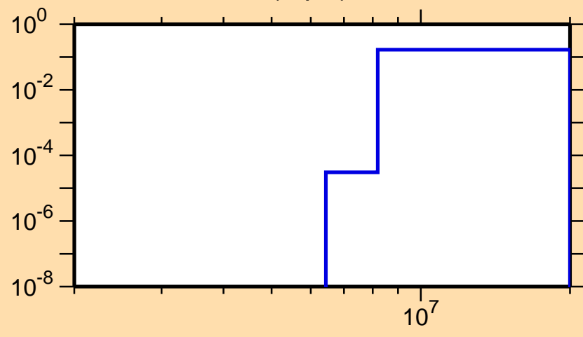
\sigma vs. E for ^{25}\text{Al}(n,p\alpha)
