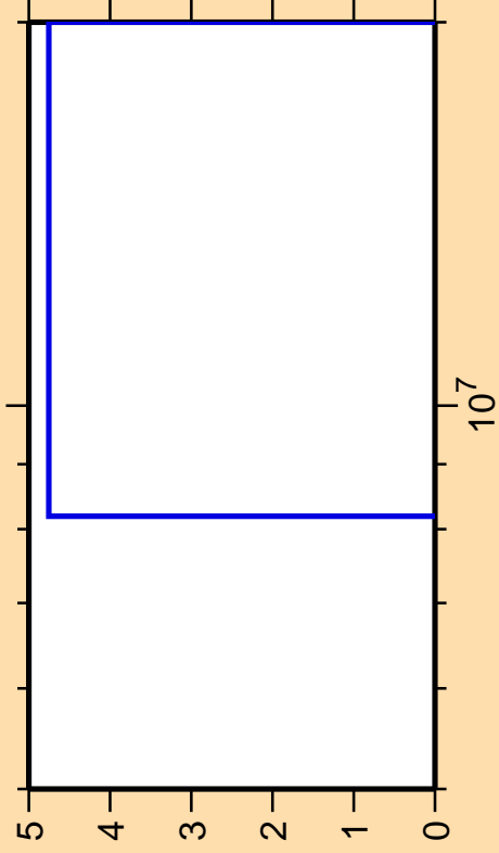
\Delta\sigma/\sigma vs. E for ^{25}\text{Al}(n,\text{pt})
