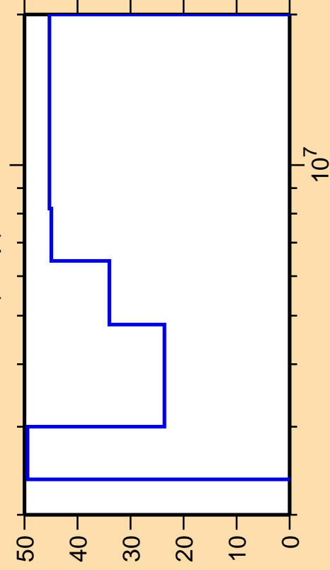
\Delta\sigma/\sigma vs. E for ^{25}\text{Al}(n,np)
