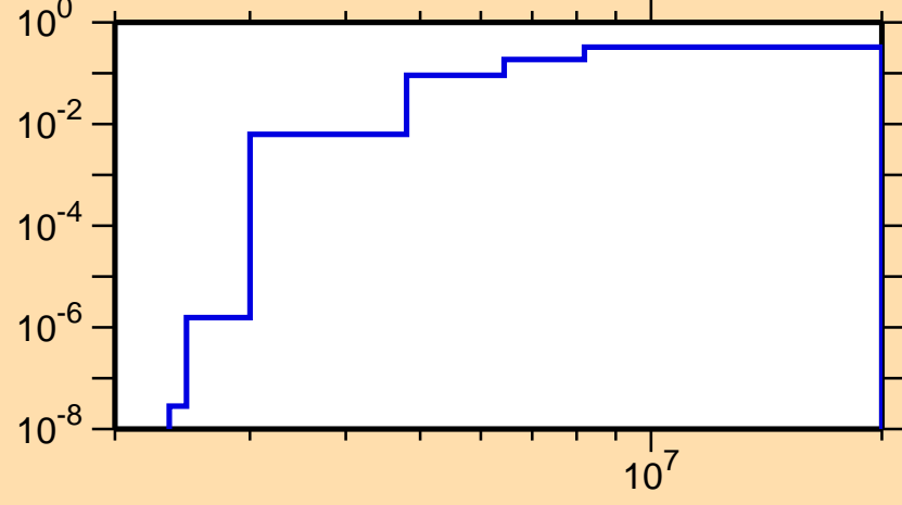
\sigma vs. E for ^{25}\text{Al}(n,np)
