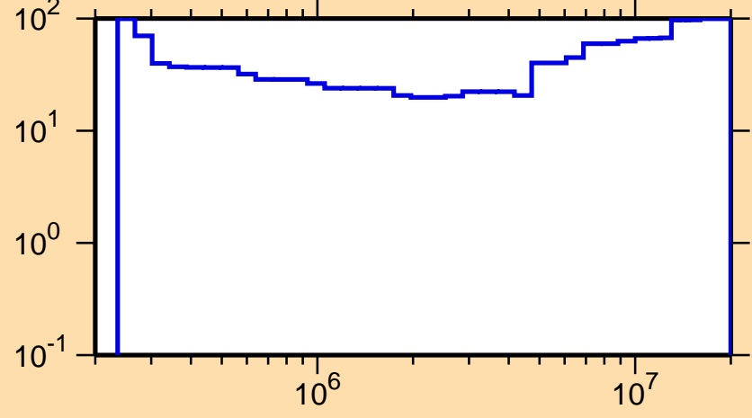
\Delta\sigma/\sigma vs. E for ^{26}\text{Al}(n,n_1)
