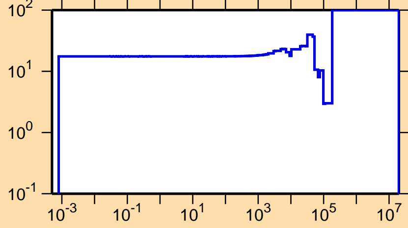
\Delta\sigma/\sigma vs. E for ^{26}\text{Al}(n,\gamma)
