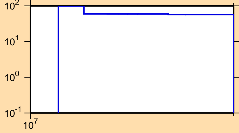
\Delta\sigma/\sigma vs. E for ^{26}\text{Al}(n,2n)
