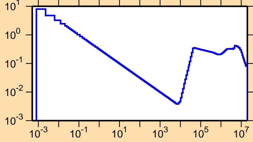
\sigma vs. E for ^{26}\text{Al}(n,p)
