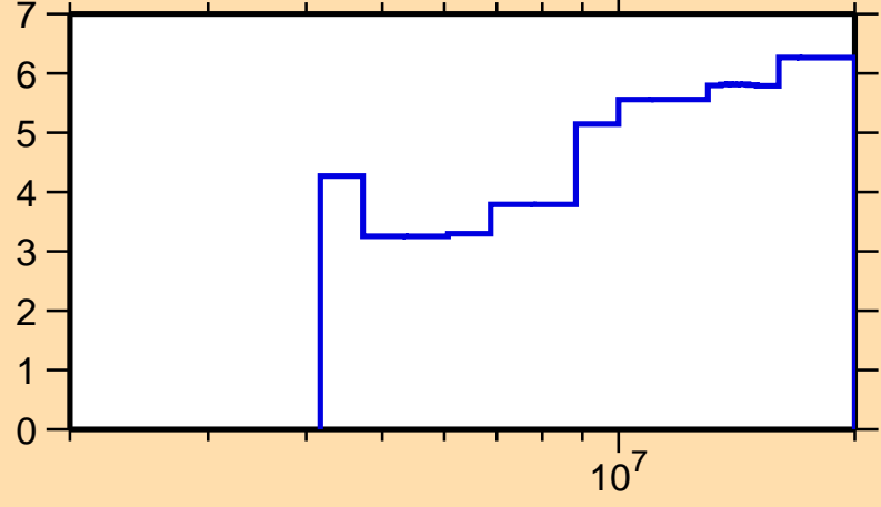
\Delta\sigma/\sigma vs. E for ^{26}\text{Al}(n,\text{nonel.})
