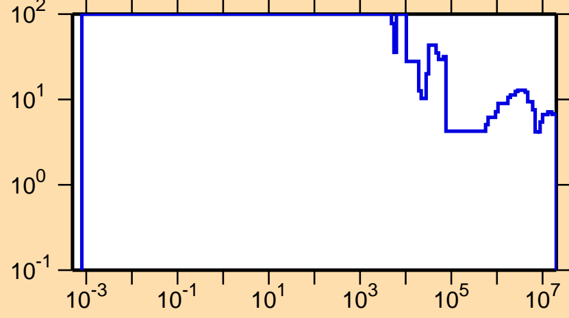
\Delta\sigma/\sigma vs. E for ^{26}\text{Al}(n,el.)
