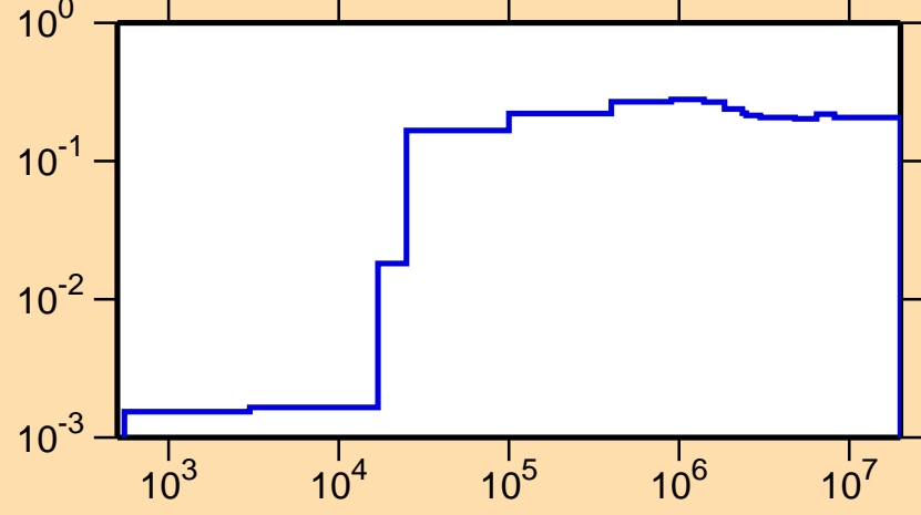
\sigma vs. E for ^{26}\text{Al}(n,\alpha)
