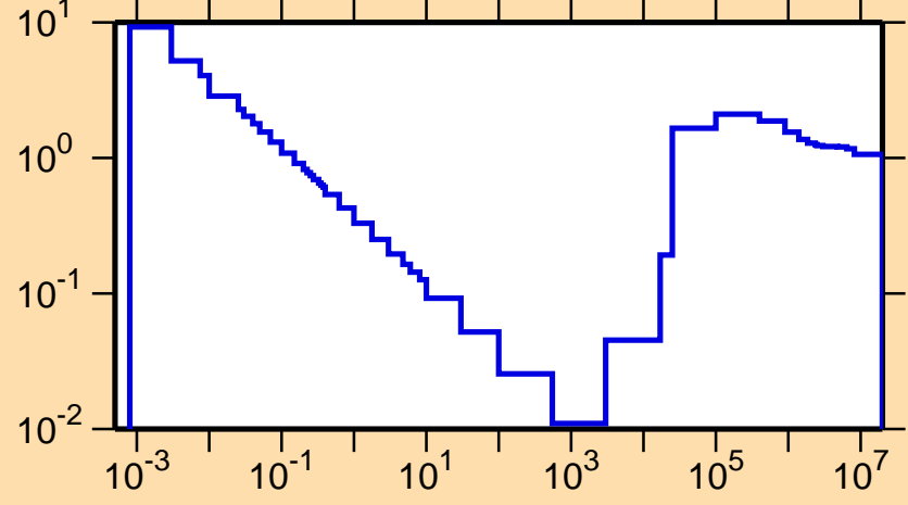
\sigma vs. E for ^{26}\text{Al}(n,\text{nonel.})
