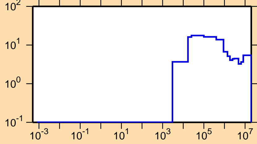
\Delta\sigma/\sigma vs. E for ^{26}\text{Al}(n,\text{nonel.})
