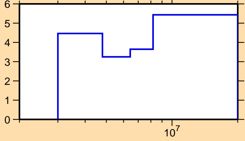
\Delta\sigma/\sigma vs. E for ^{26}\text{Al}(n,nonel.)
