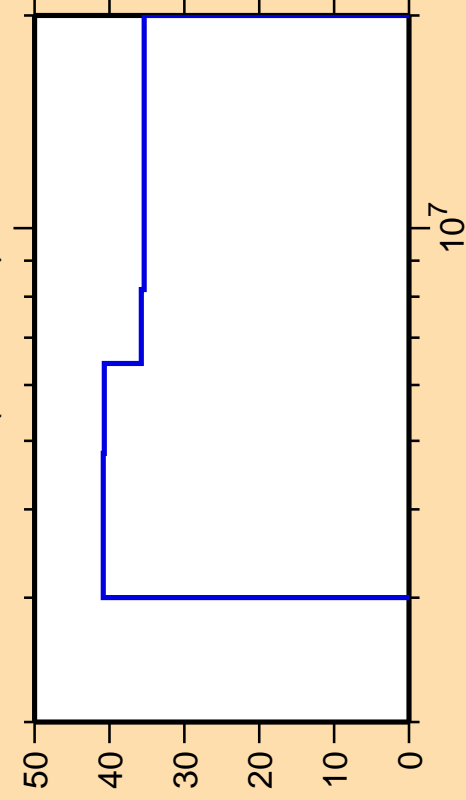
\Delta\sigma/\sigma vs. E for ^{26}\text{Al}(n,ncont.)
