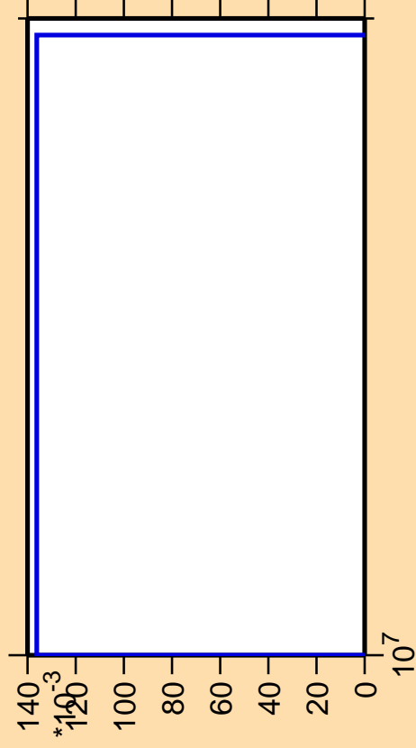
\Delta\sigma/\sigma vs. E for ^{27}\text{Al}(n,nt)
