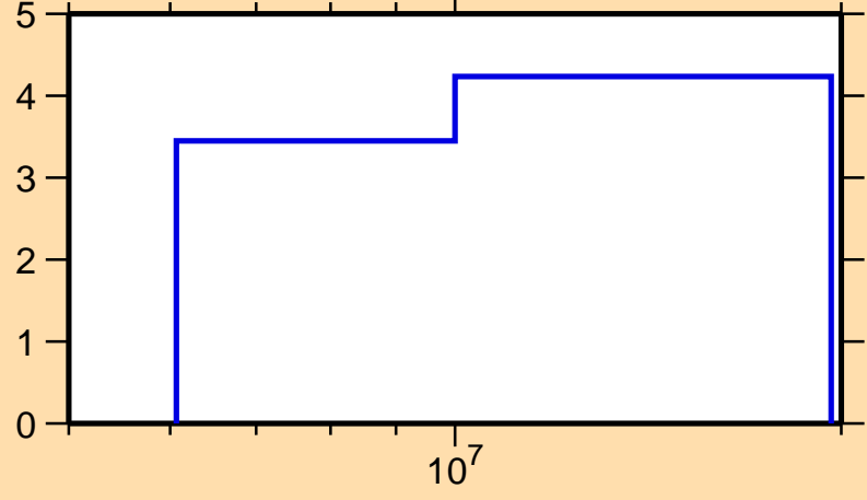
\Delta\sigma/\sigma vs. E for ^{27}\text{Al}(n,\text{tot.})
