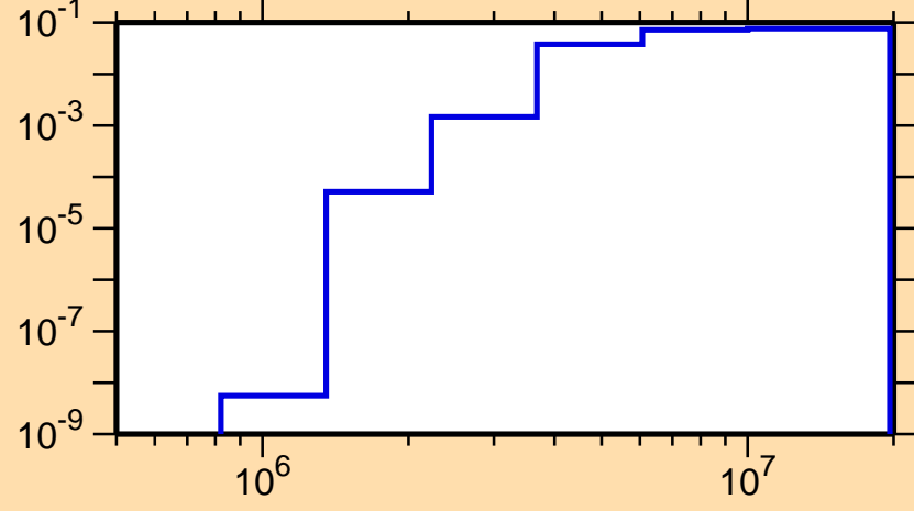
\sigma vs. E for ^{28}\text{Al}(n,p)
