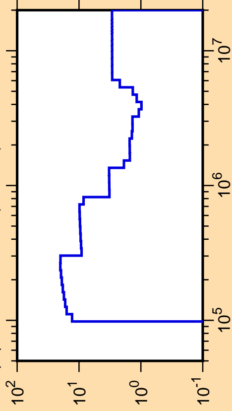
\Delta\mu/\mu vs. E for ^{29}\text{Al}(\text{mt251})
