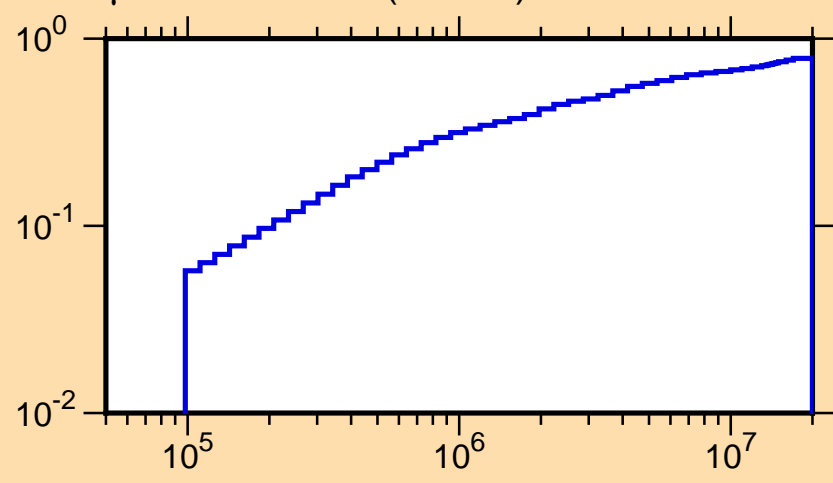
\mu vs. E for ^{29}\text{Al}(\text{mt251})
