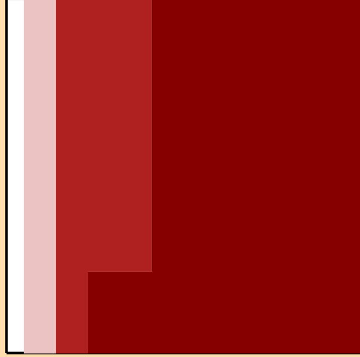
\Delta\sigma/\sigma vs. E for ^{30}\text{Al}(n,2n)
