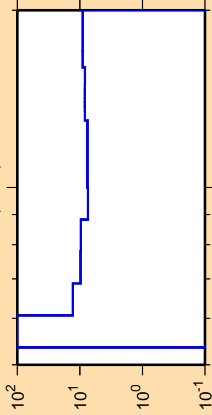
\Delta\sigma/\sigma vs. E for ^{30}\text{Al}(n,2n)
