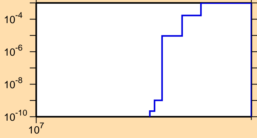
\sigma vs. E for ^{30}\text{Al}(n,\text{nd})
