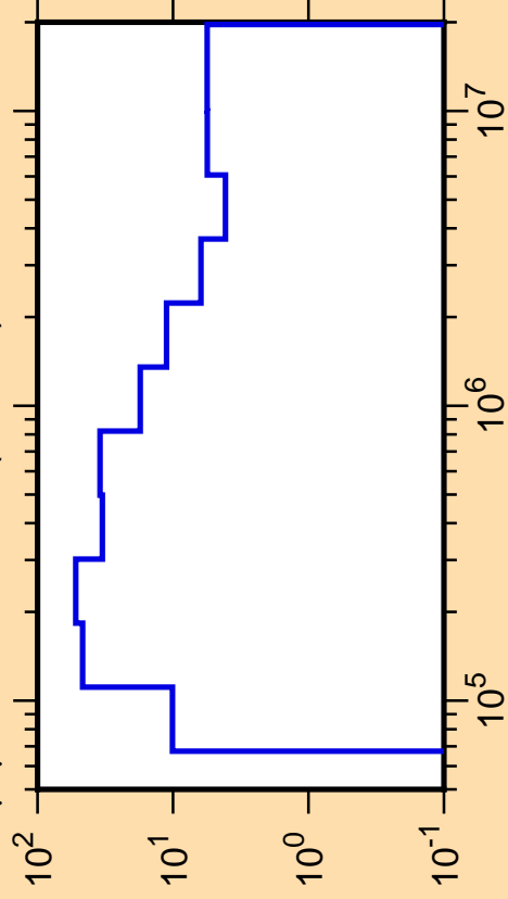
\Delta\mu/\mu vs. E for ^{30}\text{Al}(\text{mt251})
