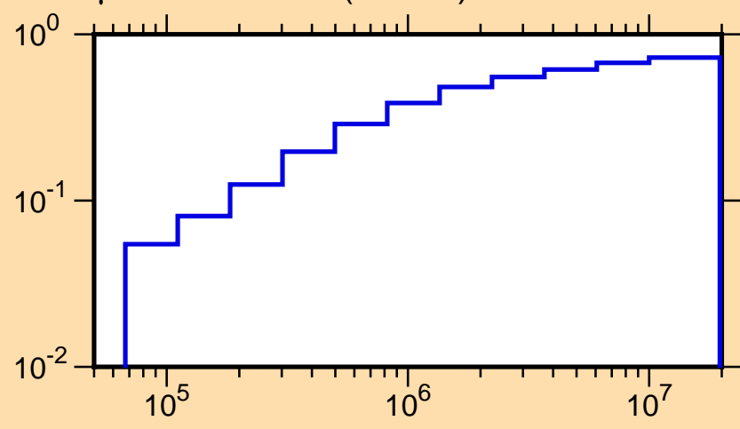
\mu vs. E for ^{30}\text{Al}(\text{mt251})
