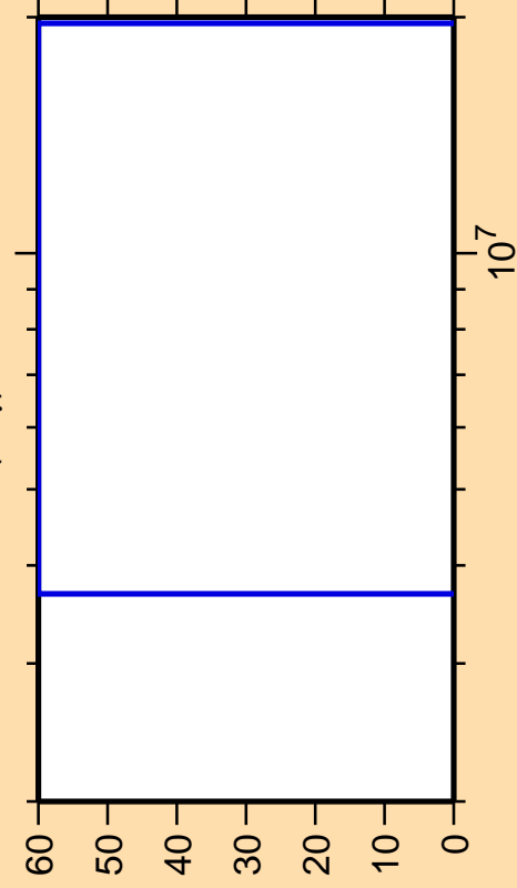
\Delta\sigma/\sigma vs. E for ^{30}\text{Al}(n,\gamma)
