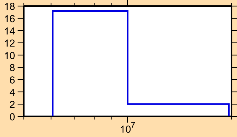
\Delta\sigma/\sigma vs. E for ^{30}\text{Al}(n,el.)
