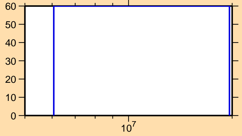
\Delta\sigma/\sigma vs. E for ^{30}\text{Al}(n,ncont.)
