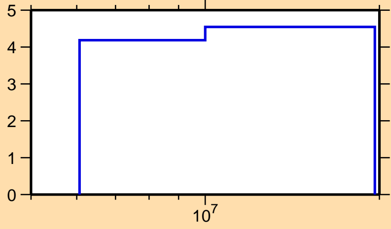
\Delta\sigma/\sigma vs. E for ^{30}\text{Al}(n,n\text{nonel.})
