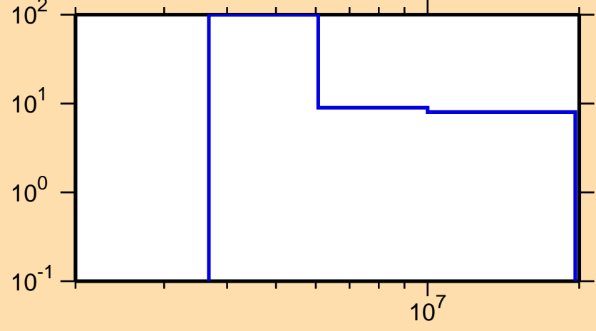
\Delta\sigma/\sigma vs. E for ^{30}\text{Al}(n,2n)
