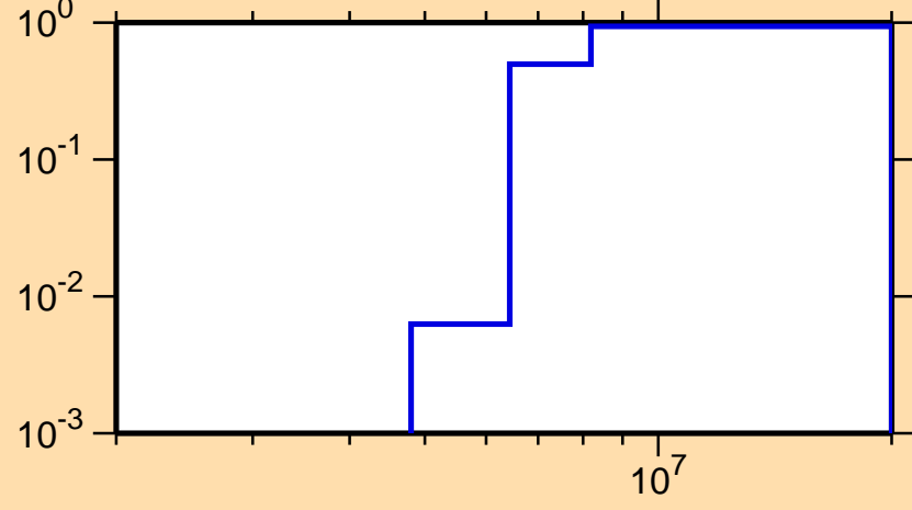
\sigma vs. E for ^{30}\text{Al}(n,2n)
