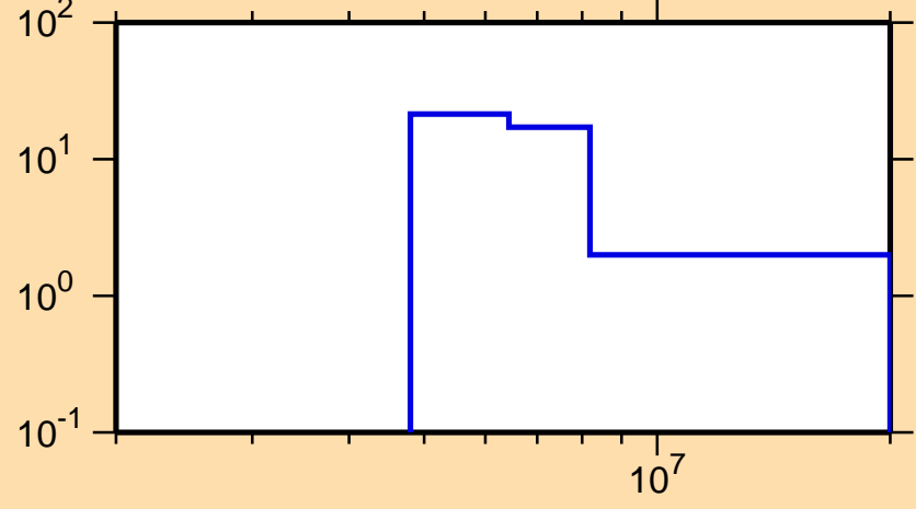
\Delta\sigma/\sigma vs. E for ^{30}\text{Al}(n,\text{el.})
