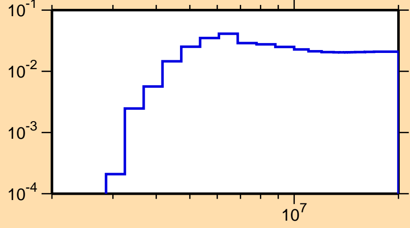
\sigma vs. E for ^{35}\text{Ar}(n,n\text{cont.})
