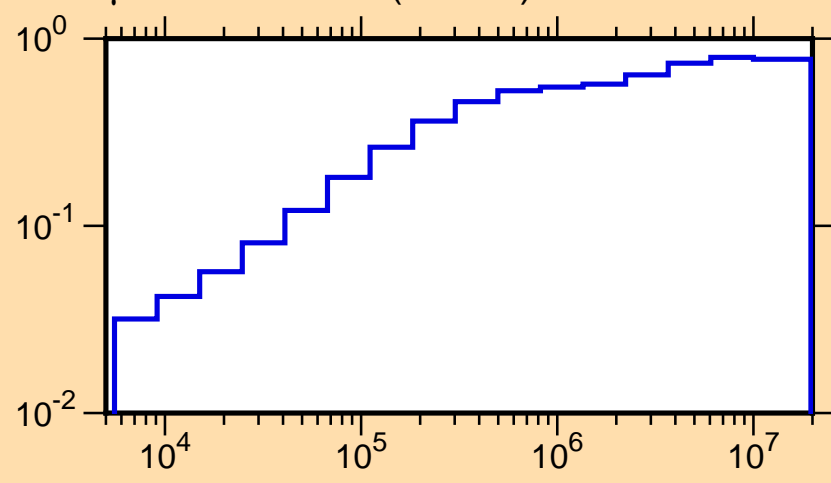
\mu vs. E for ^{35}\text{Ar}(\text{mt251})
