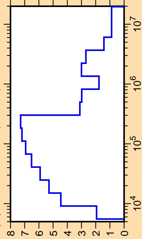
\Delta\mu/\mu vs. E for ^{35}\text{Ar}(\text{mt251})
