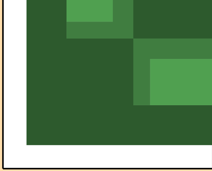
Correlation Matrix
