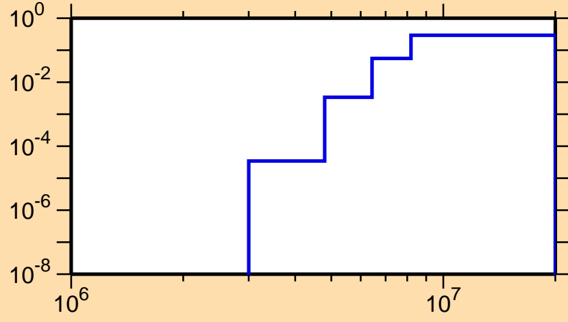
\sigma vs. E for ^{35}\text{Ar}(n,p\alpha)
