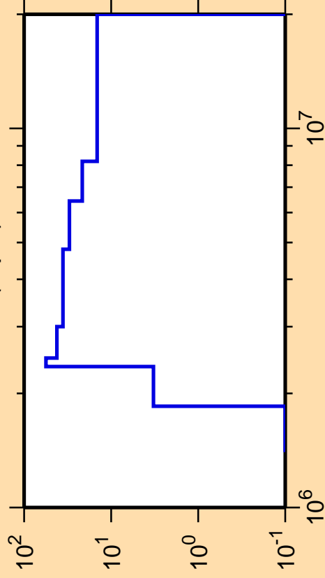
\Delta\sigma/\sigma vs. E for ^{35}\text{Ar}(n,p\alpha)
