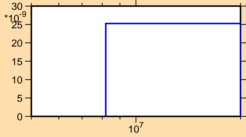
\sigma vs. E for ^{35}\text{Ar}(n,\text{nd})
