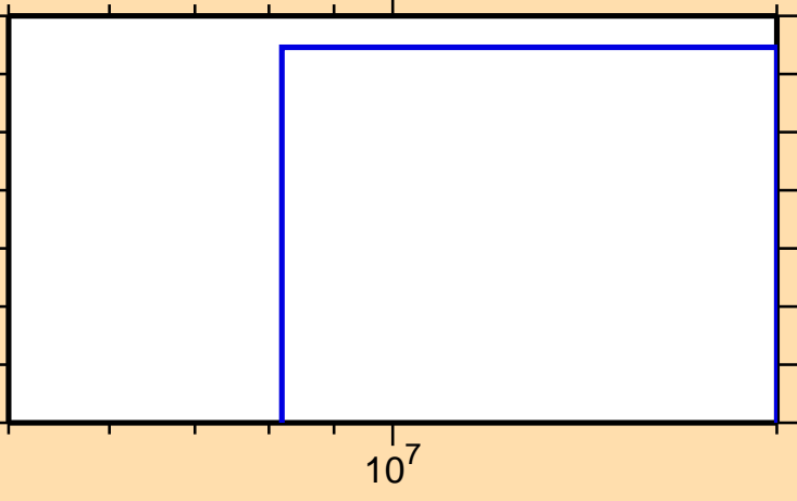
\sigma vs. E for ^{35}\text{Ar}(n,\text{pt})
