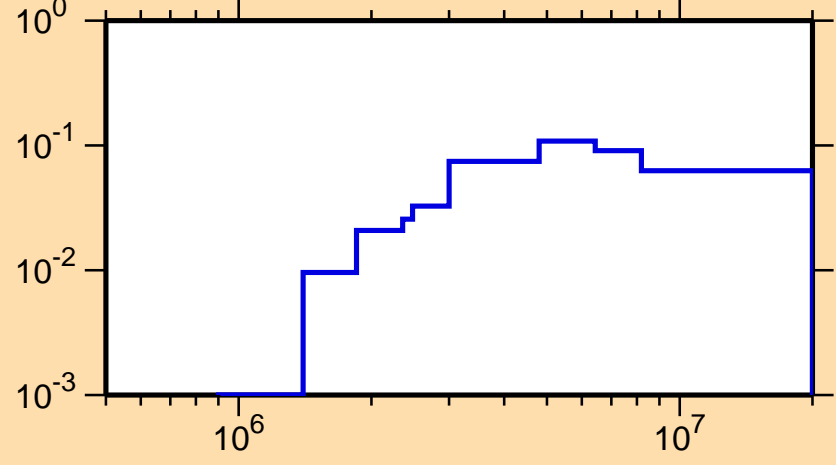
\sigma vs. E for ^{35}\text{Ar}(n,\text{inel.})
