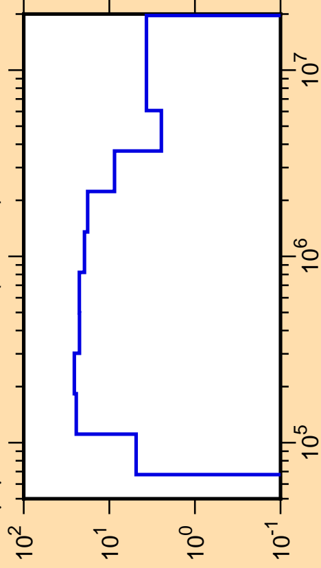
\Delta\mu/\mu vs. E for ^{36}\text{Ar}(\text{mt251})
