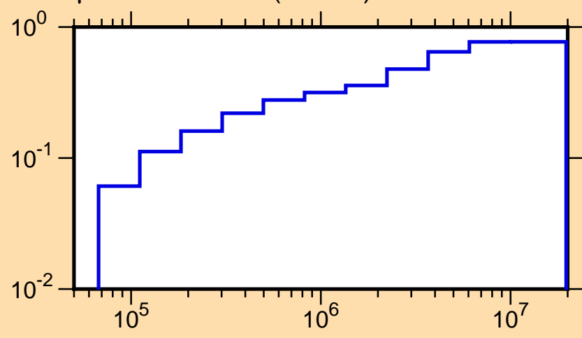
\mu vs. E for ^{36}\text{Ar}(\text{mt251})
