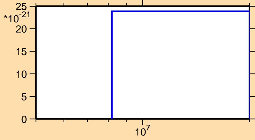
\sigma vs. E for ^{36}\text{Ar}(\text{mt } 34)
