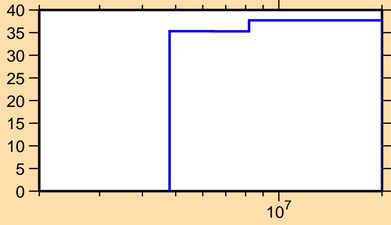
\Delta\sigma/\sigma vs. E for ^{36}\text{Ar}(n,ncont.)
