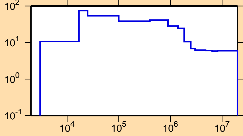
\Delta\sigma/\sigma vs. E for ^{36}\text{Ar}(n,\text{nonel.})
