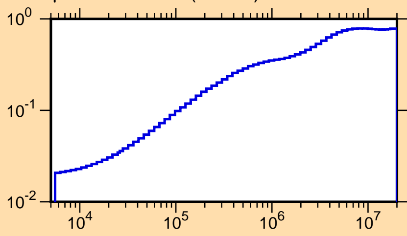
\mu vs. E for ^{37}\text{Ar}(\text{mt251})
