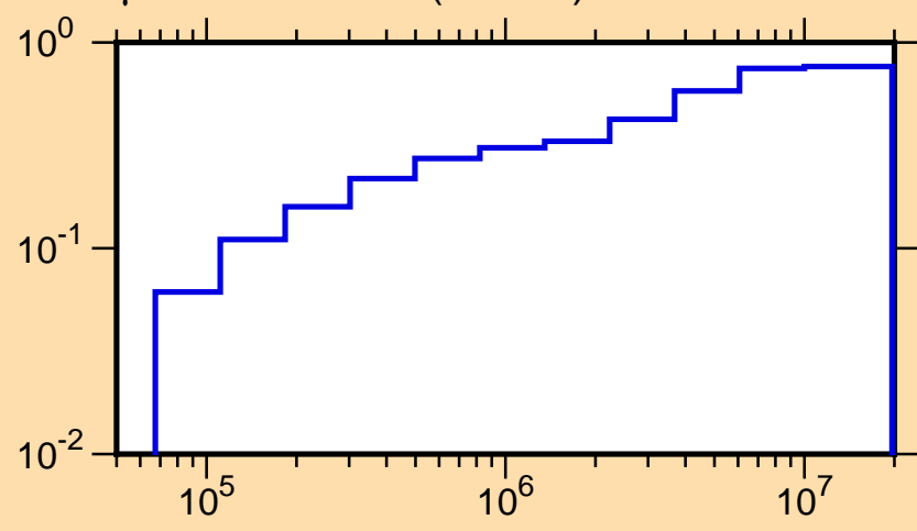
\mu vs. E for ^{38}\text{Ar}(\text{mt251})
