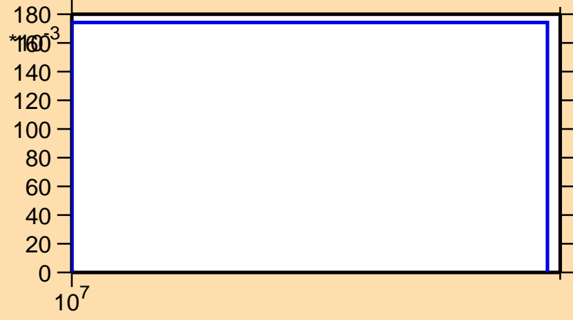
\sigma vs. E for ^{38}\text{Ar}(n,np)
