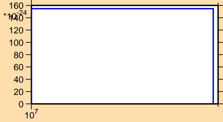
\sigma vs. E for ^{38}\text{Ar}(\text{mt } 45)
