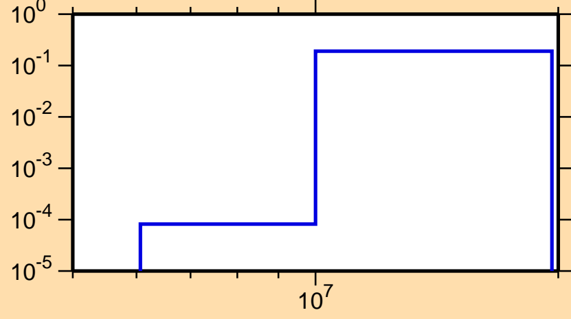
\sigma vs. E for ^{38}\text{Ar}(n,n\alpha)
