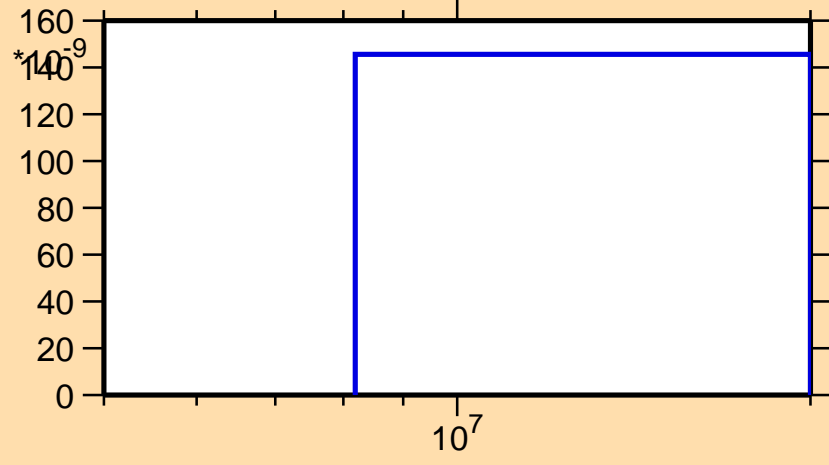
\sigma vs. E for ^{39}\text{Ar}(n,p\alpha)
