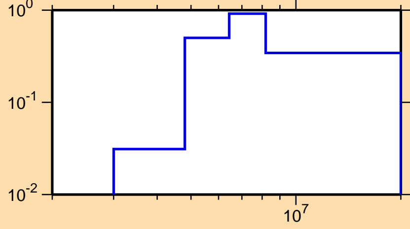
\sigma vs. E for ^{39}\text{Ar}(n,n\text{cont.})
