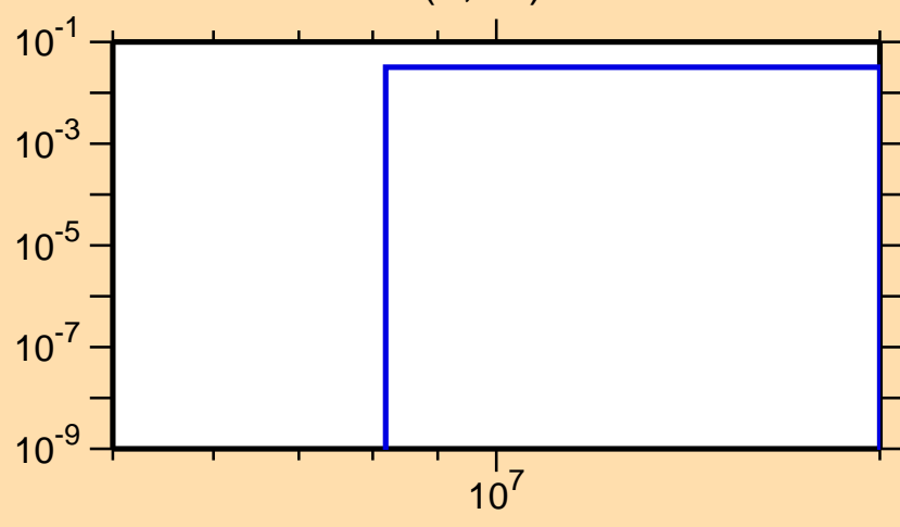
\sigma vs. E for ^{39}\text{Ar}(n,\alpha)
