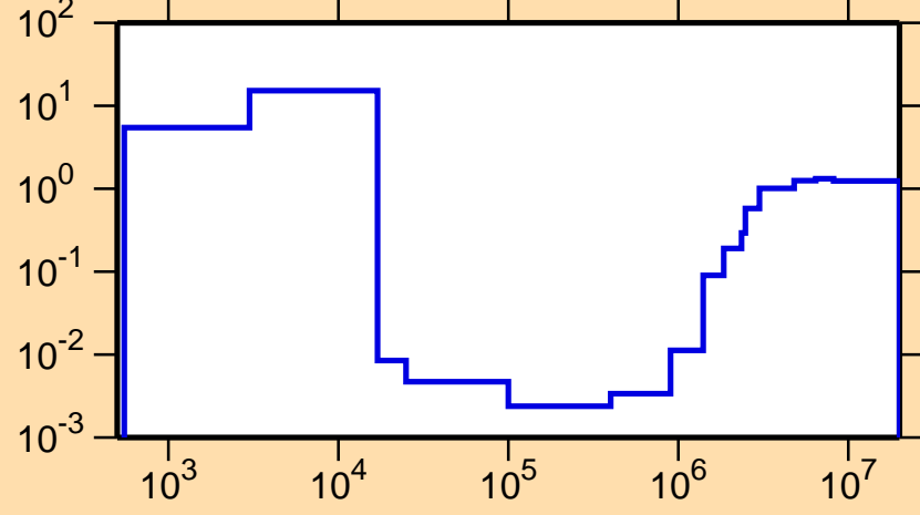
\sigma vs. E for ^{39}\text{Ar}(n,\text{nonel.})
